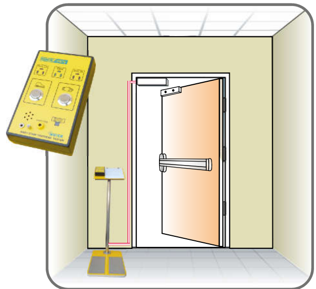
This Combo Tester can be connected to Door Control System thru Access Control System Signal from this Tester. It gives signal of \pm 400V (Peak DC/AC); 100mA to operate relay (KAQW214) of Access Control System
