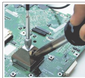
HAP 200 Hot Air Pencil with WRK Nozzle
