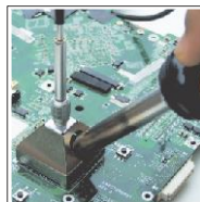
Large SMD Desoldering
