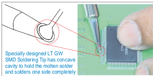
WP 80 Soldering Pencil with SMD soldering tip
